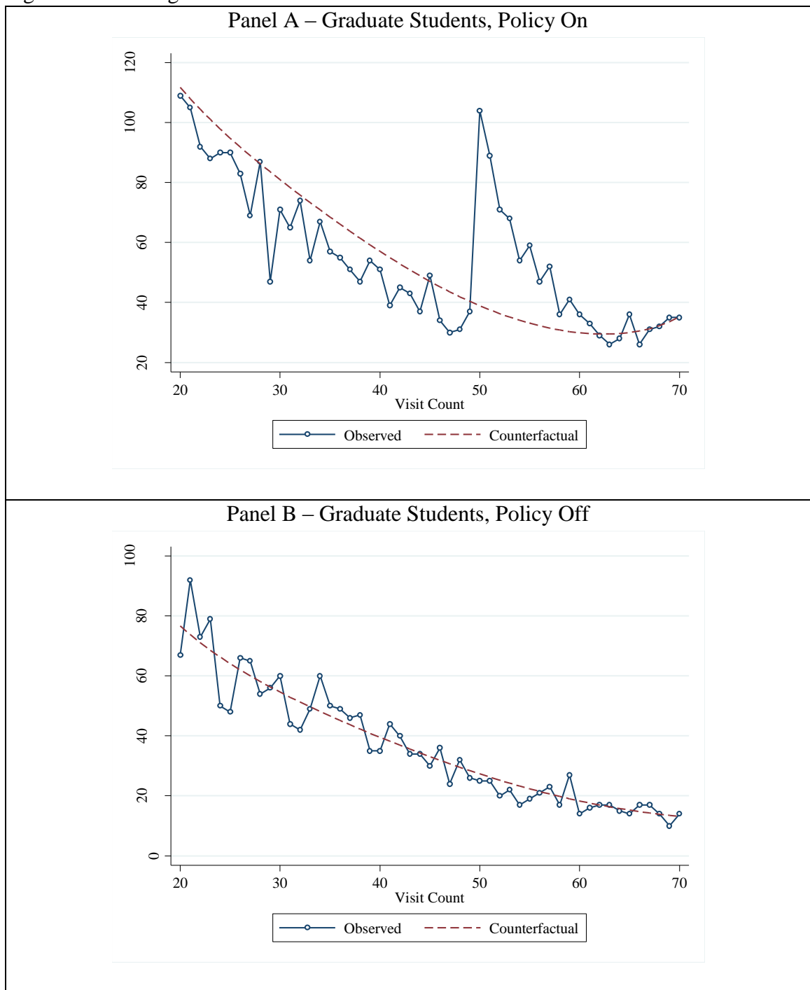
Figure 2: Bunching Estimation
